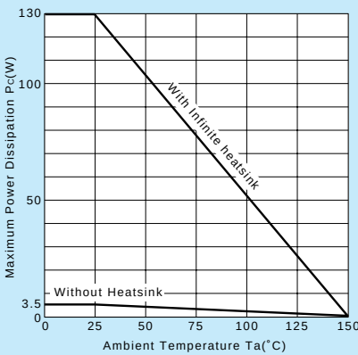
PC-Ta Derating
