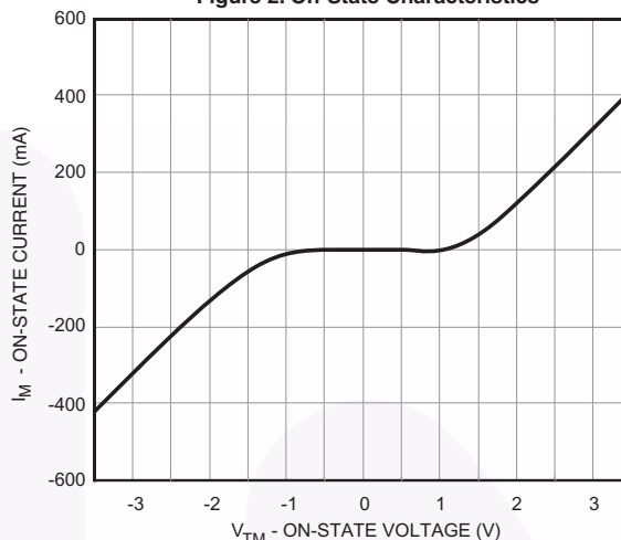
Figure 2. On-State Characteristics
