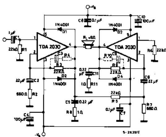
Figure 17. Bridge amplifier configuration with split power supply ( P_0 = 28W , V_s = \pm 14V )
