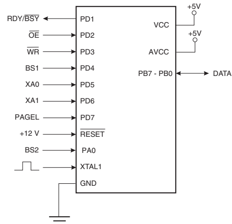
Figure 127. Parallel Programming
