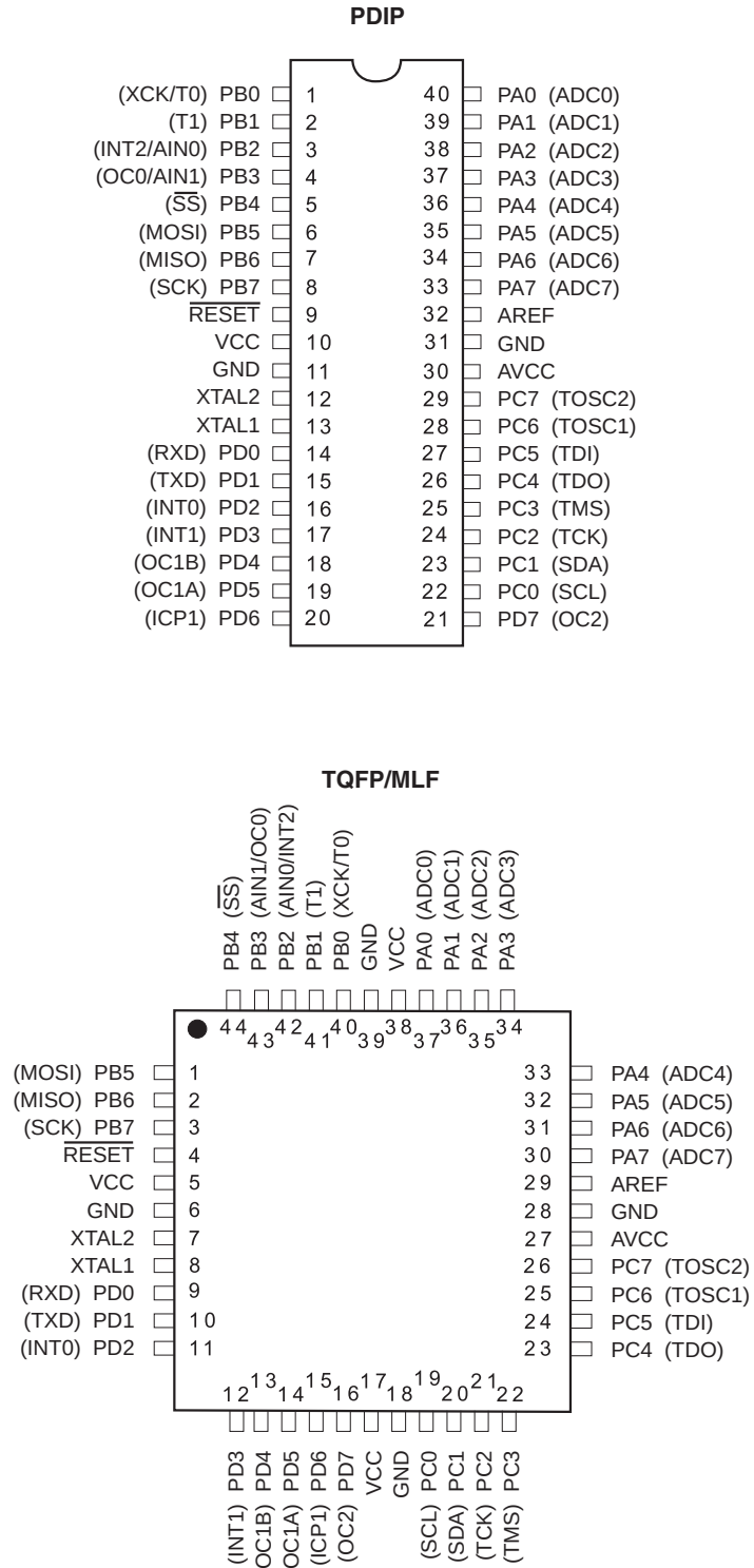
Figure 1. Pinout ATmega32
