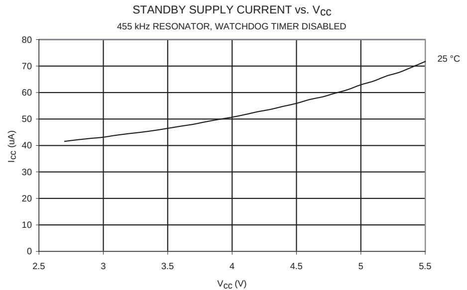
Figure 170. Standby Supply Current vs. V_{CC} (455 kHz Resonator, WDT Disabled)
