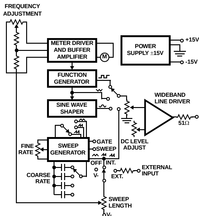
FIGURE 10D. INTERCONNECTIONS
