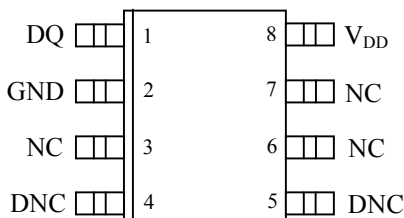
DS1821S 8-Pin SOIC (208-mil) See Mech Drawings Section
