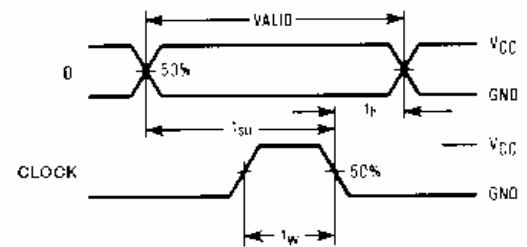
Figure 4. Switching Waveforms
