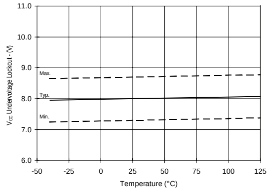
Figure 26. V_{CC} Undervoltage Lockout (-) vs. Temperature
