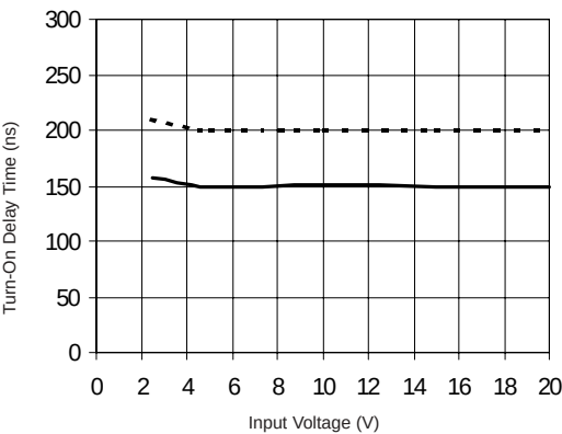
Figure 32A. Turn-On Time vs. Input Voltage
