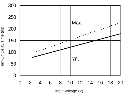
Figure 32B. Turn-Off Time vs. Input Voltage
