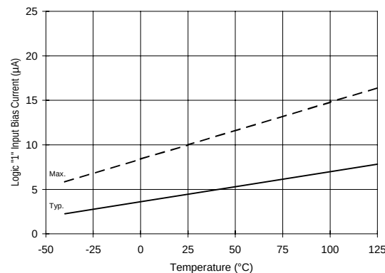
Figure 23A. Logic "1" Input Current vs. Temperature
