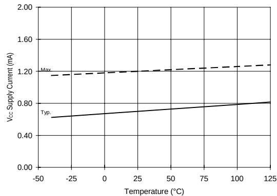
Figure 22A. V CC Supply Current vs. Temperature
