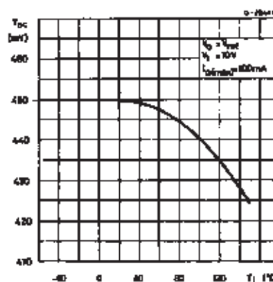
Figure 18. Current Limit Sense Voltage vs. Junction Temperature.
