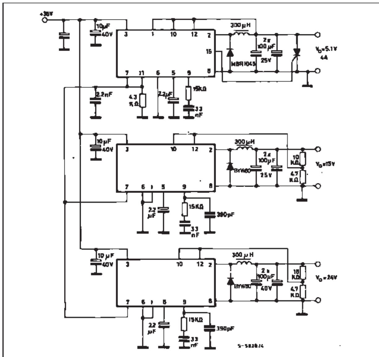
The Synchronization of the Three L296s.
