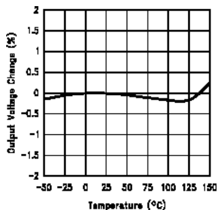
Temperature Stability
