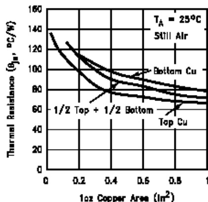
FIGURE 7. \theta_{JA} vs. 1oz Copper Area for SOT-223
