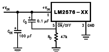
FIGURE 14. Delayed Startup
