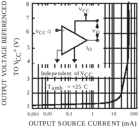
OUTPUT CHARACTERISTICS
