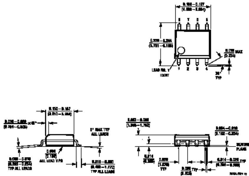
8-Lead Surface Mount Package (M) Order Number LM2931AM-5.0, LM2931M-5.0 or LM2931CM NS Package Number M08A
