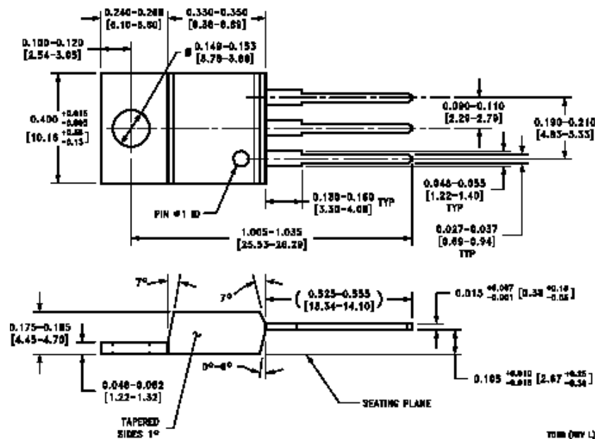
3-Lead TO-220 Plastic Package (T) Order Number LM2931AT-5.0 or LM2931T-5.0 NS Package Number T03B
