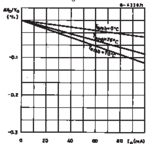
Figure 4 : Load Regulation Characteristics without Current Limiting.
