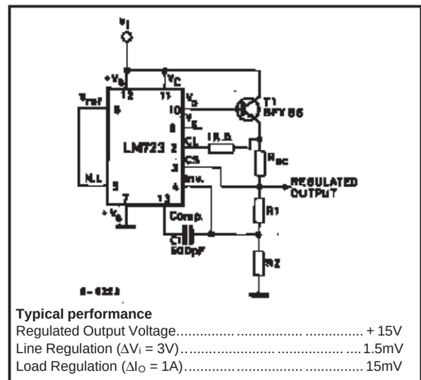
Figure 16 : Positive Voltage Regulator (external
